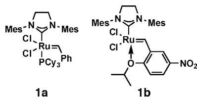
Figure 1. Metathesis catalysts.
